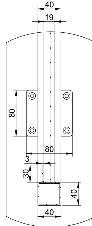
D (1:4)
